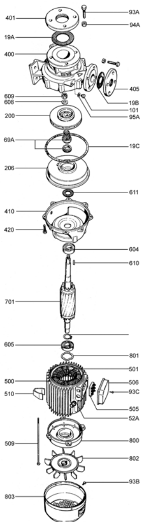
DESPIECE - A
