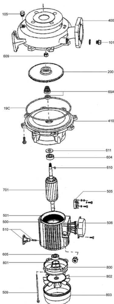
DESPIECE - B
