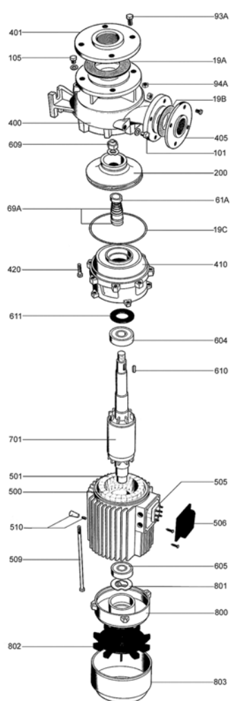
DESPIECE - C
